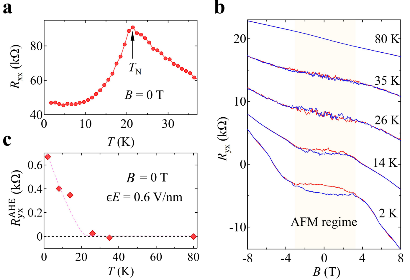
Extended Data Fig. 4 | Temperature-dependent measurements of 6SL MnBi 2 Te 4 . a , Temperature-dependent R_{xx} data showing the Néel temperature T_N . b , R_{yx} versus B measurements at different temperatures. Data at different
