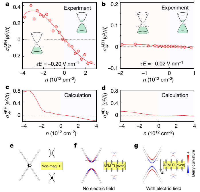
Fig. 3 | Charge-density dependence of the layer Hall effect and the layer-locked Berry curvature. a, b , The layer Hall effect as a function of charge density n with the electric field fixed at \epsilon E = -0.20 \text{ V nm}^{-1} ( a ) and \epsilon E = -0.02 \text{ V nm}^{-1} ( b ). c, d , First-principles calculated AHE conductivity \sigma_{xy}^{\text{AHE}} as a function of charge density. The theoretically applied electric field ( E^{\text{THY}} ) here can be related to the displacement field by D^{\text{THY}} = \epsilon_{\text{MnBi}_2\text{Te}_4} E^{\text{THY}} . e–g , A microscopic picture for the layer Hall effect in 6SL antiferromagnetic \text{MnBi}_2\text{Te}_4 . e , A non-magnetic topological insulator (TI) features massless surface Dirac fermions on its top and bottom layers. f , The inclusion of the A-type antiferromagnetic order gaps the Dirac fermions. The resulting Berry curvature of the top Dirac fermion exactly cancels that of the bottom Dirac fermion. g , Applying an electric field can break the degeneracy between the top and bottom Dirac fermions, leading to a large, layer-polarized AHE, as long as the Fermi level is away from the bandgap. This electric-field-induced AHE serves as the key evidence for the layer Hall effect and the layer-locked Berry curvature.
