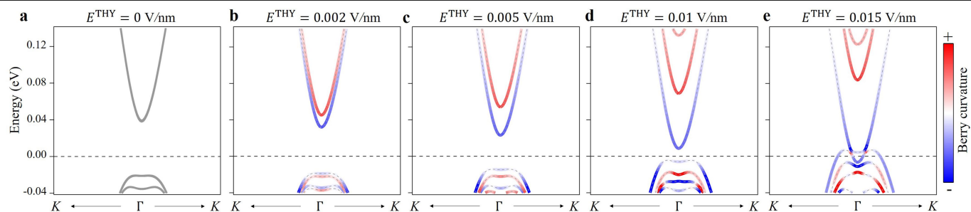
Extended Data Fig. 6 | First-principles calculated band structures. a–e , Calculated band structures of 6SL antiferromagnetic \text{MnBi}_2\text{Te}_4 for different theoretical electric fields E^{\text{THY}} .
