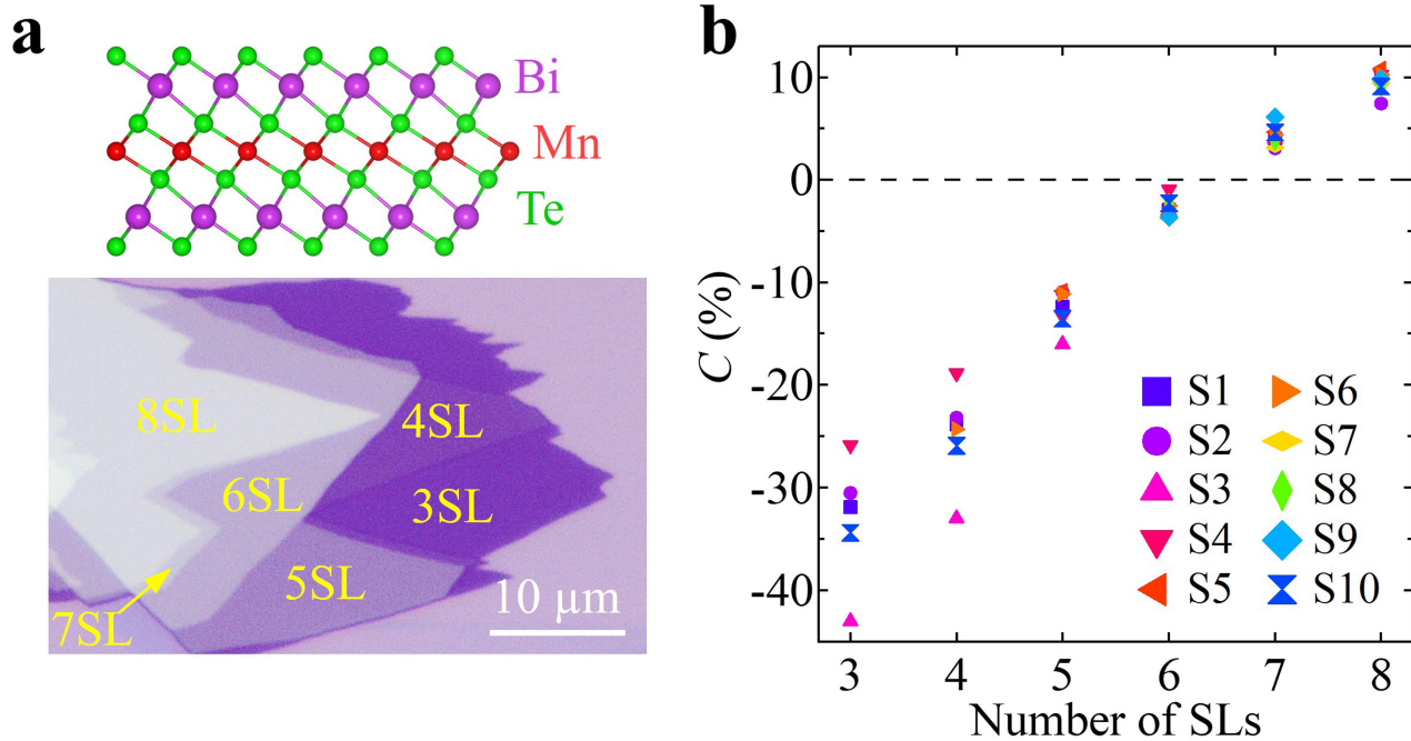
Extended Data Fig. 7 | Optical contrast of the \text{MnBi}_2\text{Te}_4 flakes. a , Lower panel, optical image of few-layer flakes of \text{MnBi}_2\text{Te}_4 exfoliated on \text{SiO}_2 substrate. Upper panel, lattice of one SL \text{MnBi}_2\text{Te}_4 . b , Optical contrast C = (I_{\text{flake}} - I_{\text{substrate}}) / (I_{\text{flake}} + I_{\text{substrate}}) as a function of number of layers, which was independently determined by atomic force microscope. This process was
