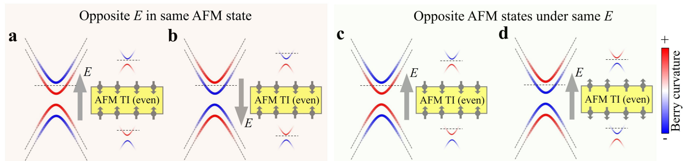
Extended Data Fig. 5 | Schematic electronic structure and Berry curvature of even-layered \text{MnBi}_2\text{Te}_4 . a, b , Same antiferromagnetic state under opposite electric fields. c, d , Opposite antiferromagnetic states under the same electric field.
